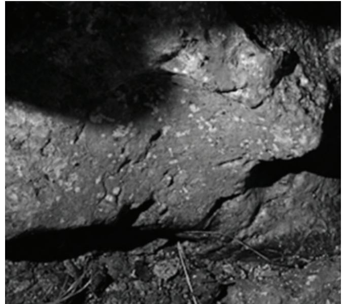
Fig. 3. Wall of Vapor cave showing the Scytonema julianum mat.
